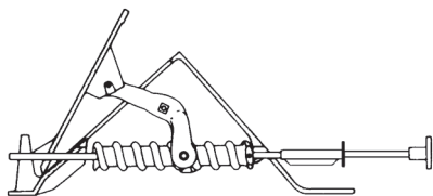
ROTARY CONTROL
